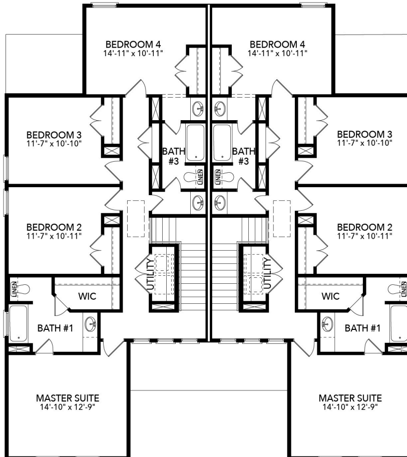
Second Floor
