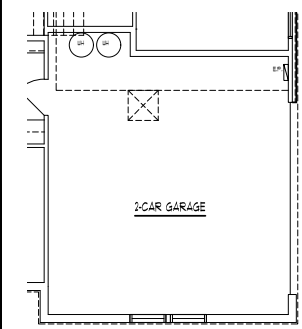
OPTIONAL 2 CAR SIDE ENTRY GARAGE FIRST FLOOR PLAN
