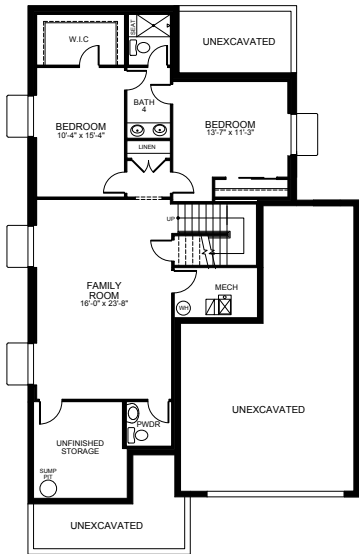
OPTIONAL FULL FINISHED BASEMENT
