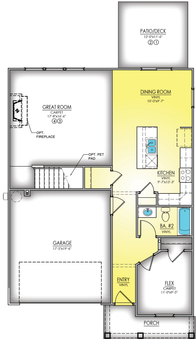
MAIN LEVEL - ELEVATION B & C
