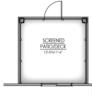
2 - OPT COVERED PATIO/DECK
