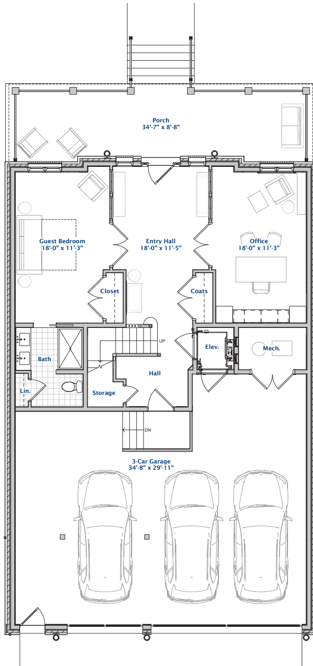
First Floor 56'-0" x 36'-8"
