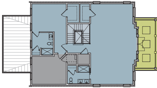
Fourth Floor 46'-3" x 36'-8"
