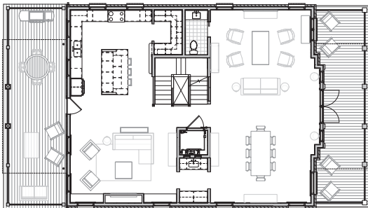
Second Floor 46'-3" x 36'-8"
