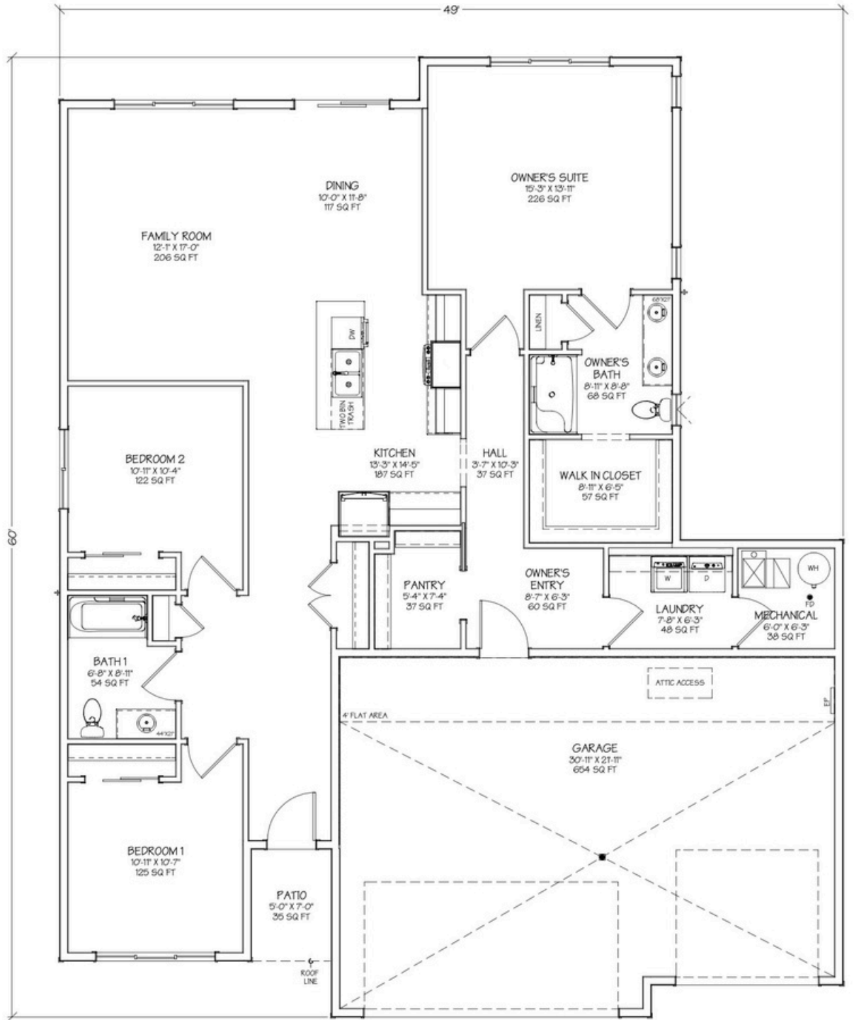
Dutton 3.0 - Base Plan - Main Floor - 1,765 sq ft
