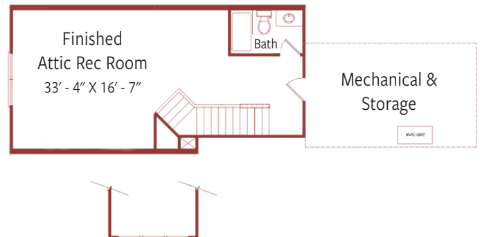
Optional Finished Attic & Optional Finished Attic Bath
