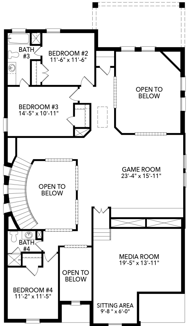
Second Floor
