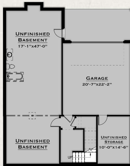
Basement Floor
