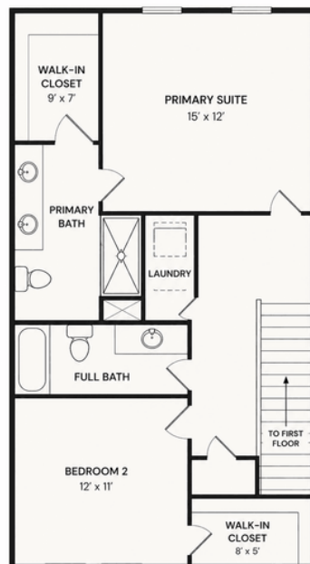
— The Belmont — Second Floor - 767 SF Room Sizes and Square Footage Are Approximate
