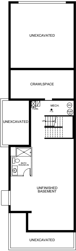
OPT. UNFINISHED BASEMENT
