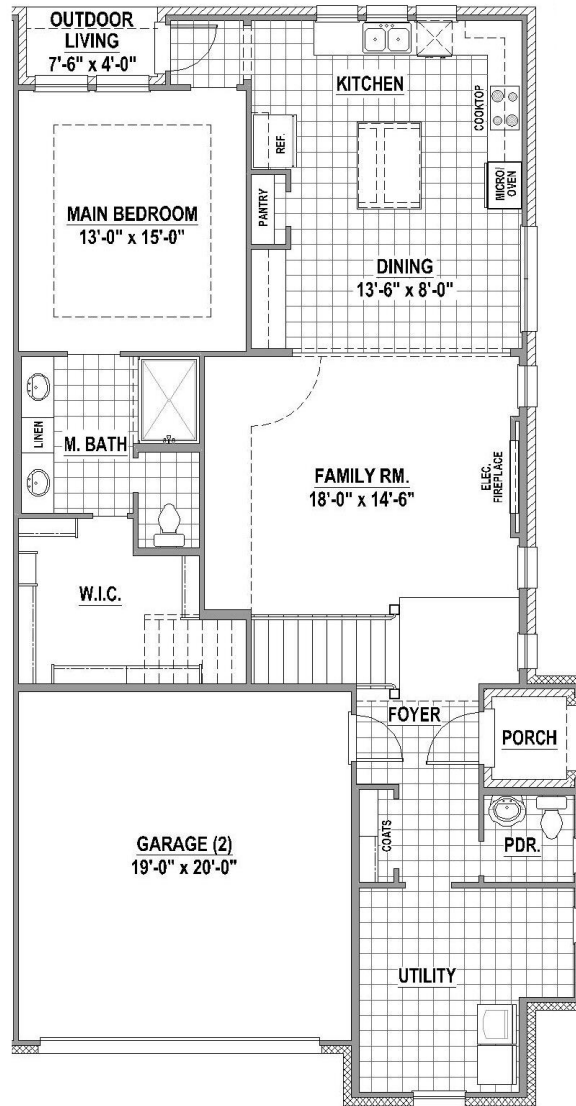
1 st Floor
