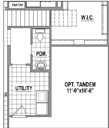
Utility & Powder Bath Configuration w/ Stairs
