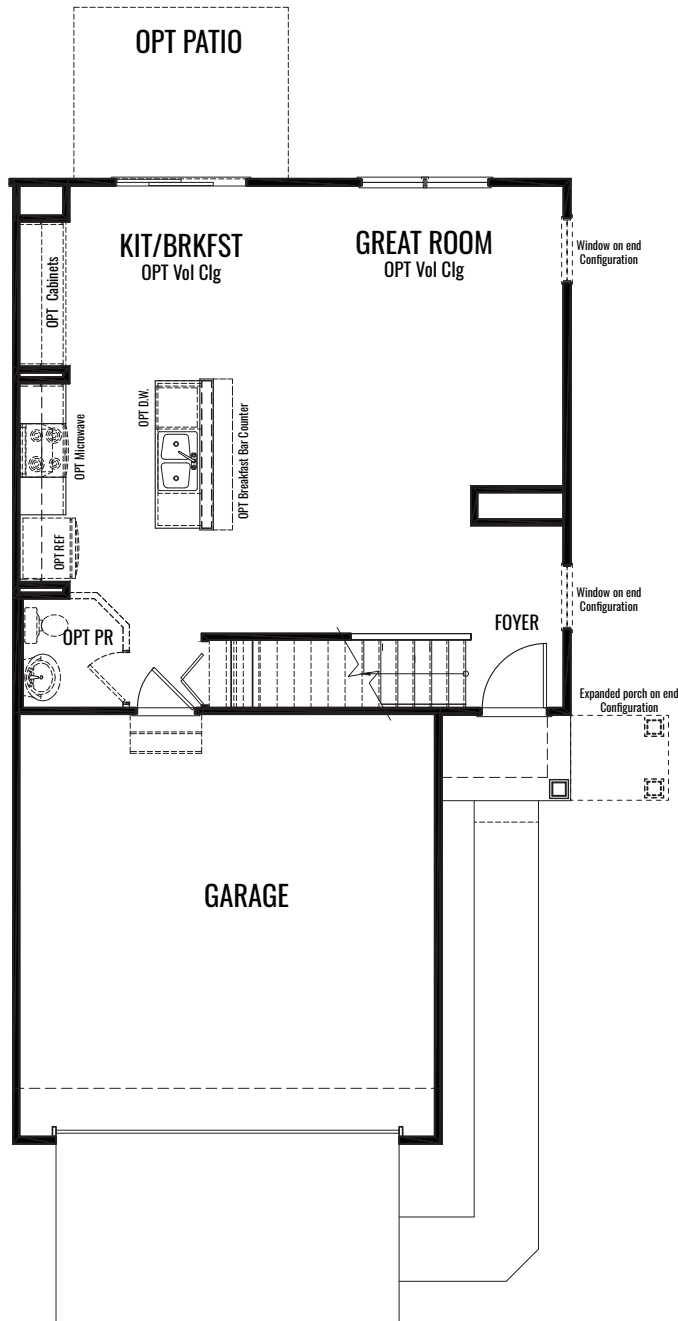
FIRST FLOOR
