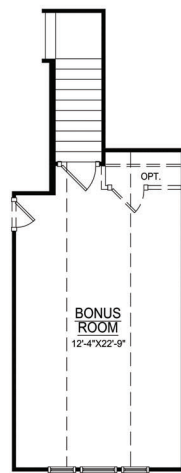
OPT. BONUS FLOOR PLAN #1
