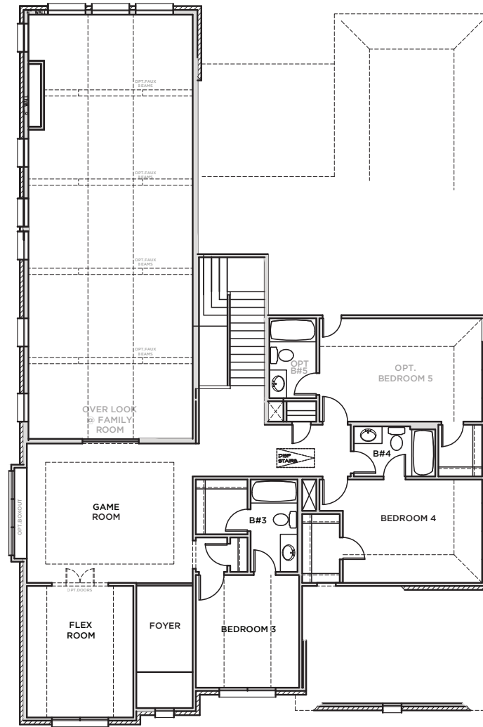
SECOND FLOOR
