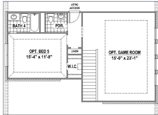
Game Room, Powder Bath & Bedroom 5 w/ Bath 4 (+791 SF)
