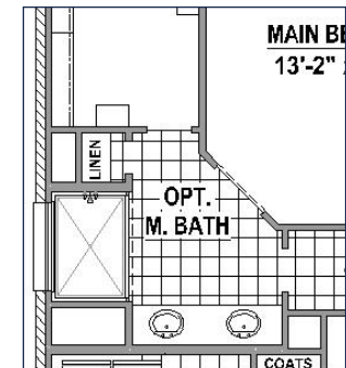
Alternate Main Bath Layout
