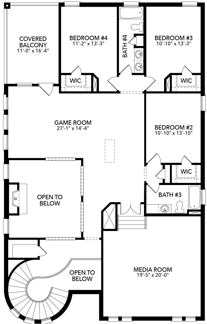
Second Floor
