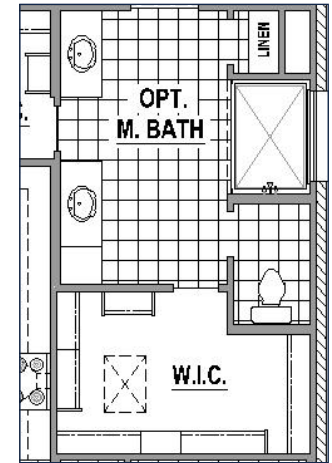
Optional Main Bath Layout (+0 SF)
