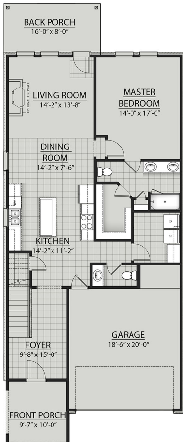
FIRST FLOOR
