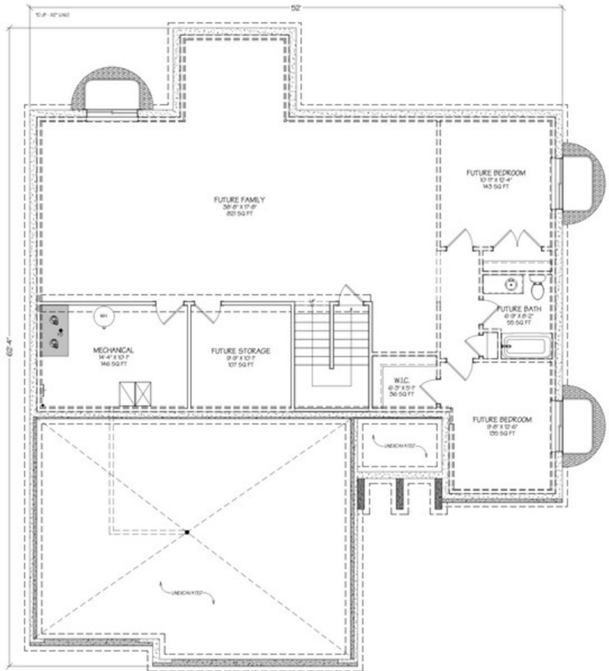
Sienna 3.0 - Base Plan - Lower Floor - 1,750 sq ft
