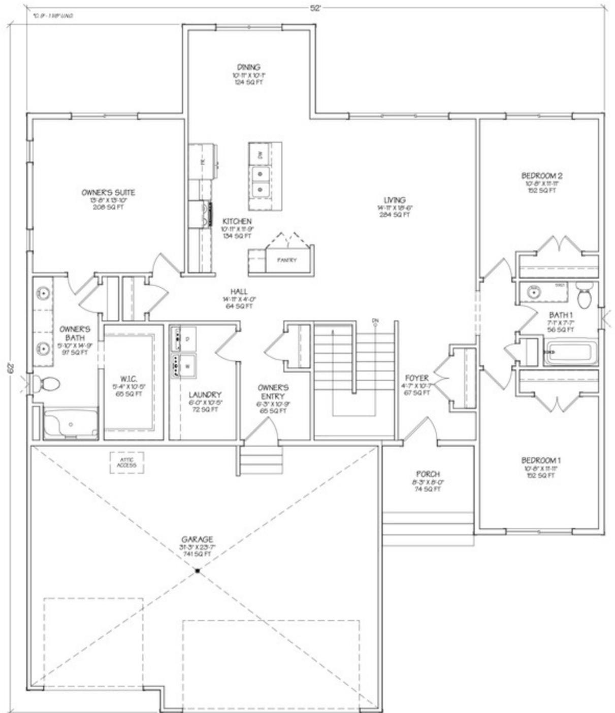
Sienna 3.0 - Base Plan - Upper Floor - 1,750 sq ft
