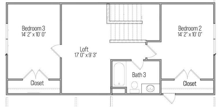
OPTIONAL SECOND FLOORPLAN
