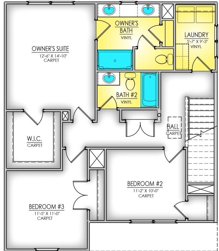
SECOND LEVEL
