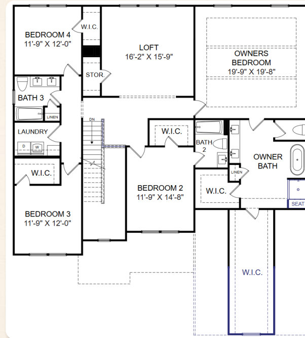
SECOND-FLOOR PLAN
