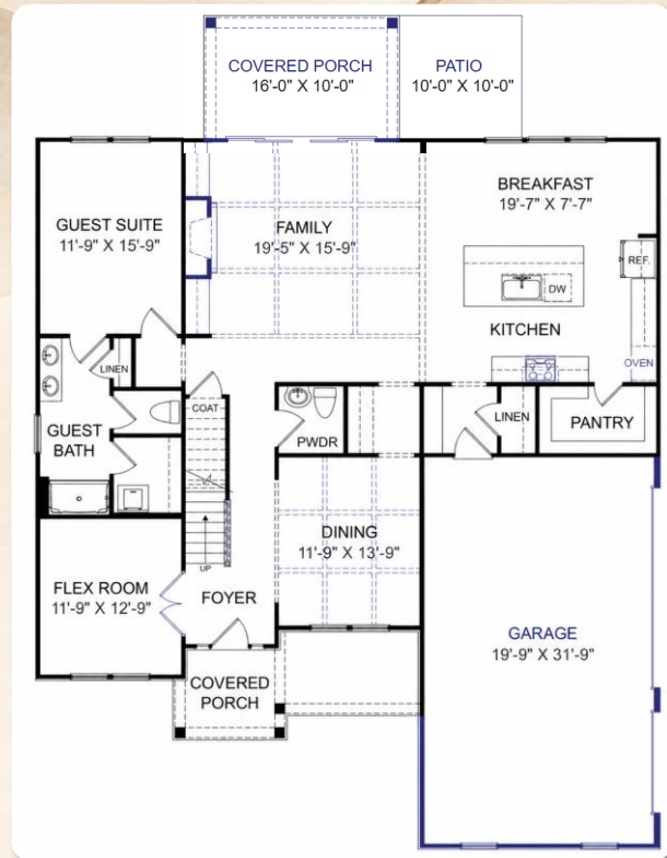
FIRST-FLOOR PLAN
