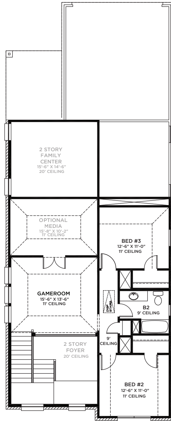
SECOND FLOOR
