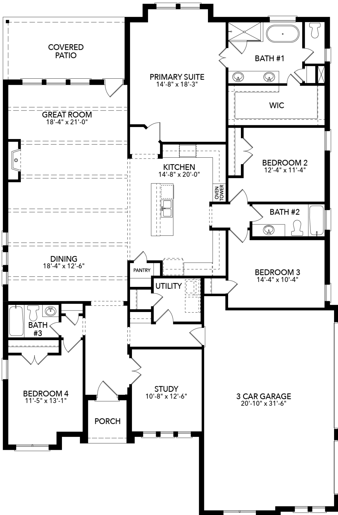
First Floor
