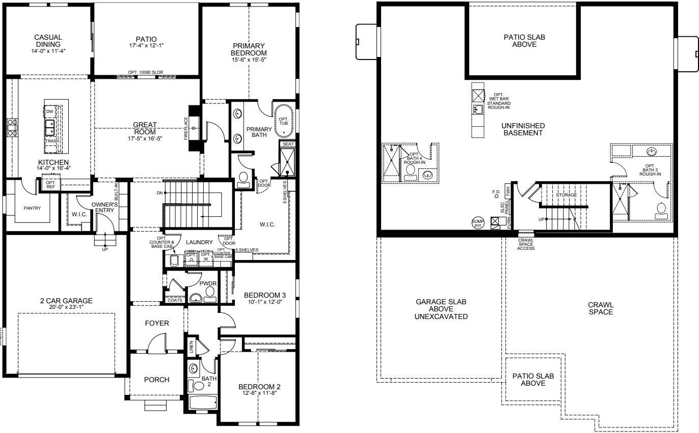
FIRST FLOOR
