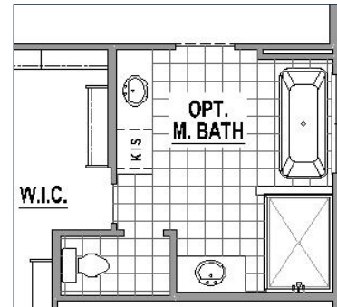
Optional Main Bath Layout
