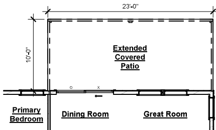
Covered Patio Extension
