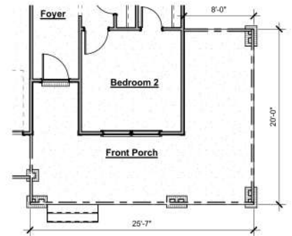
Wrap Around Front Porch
