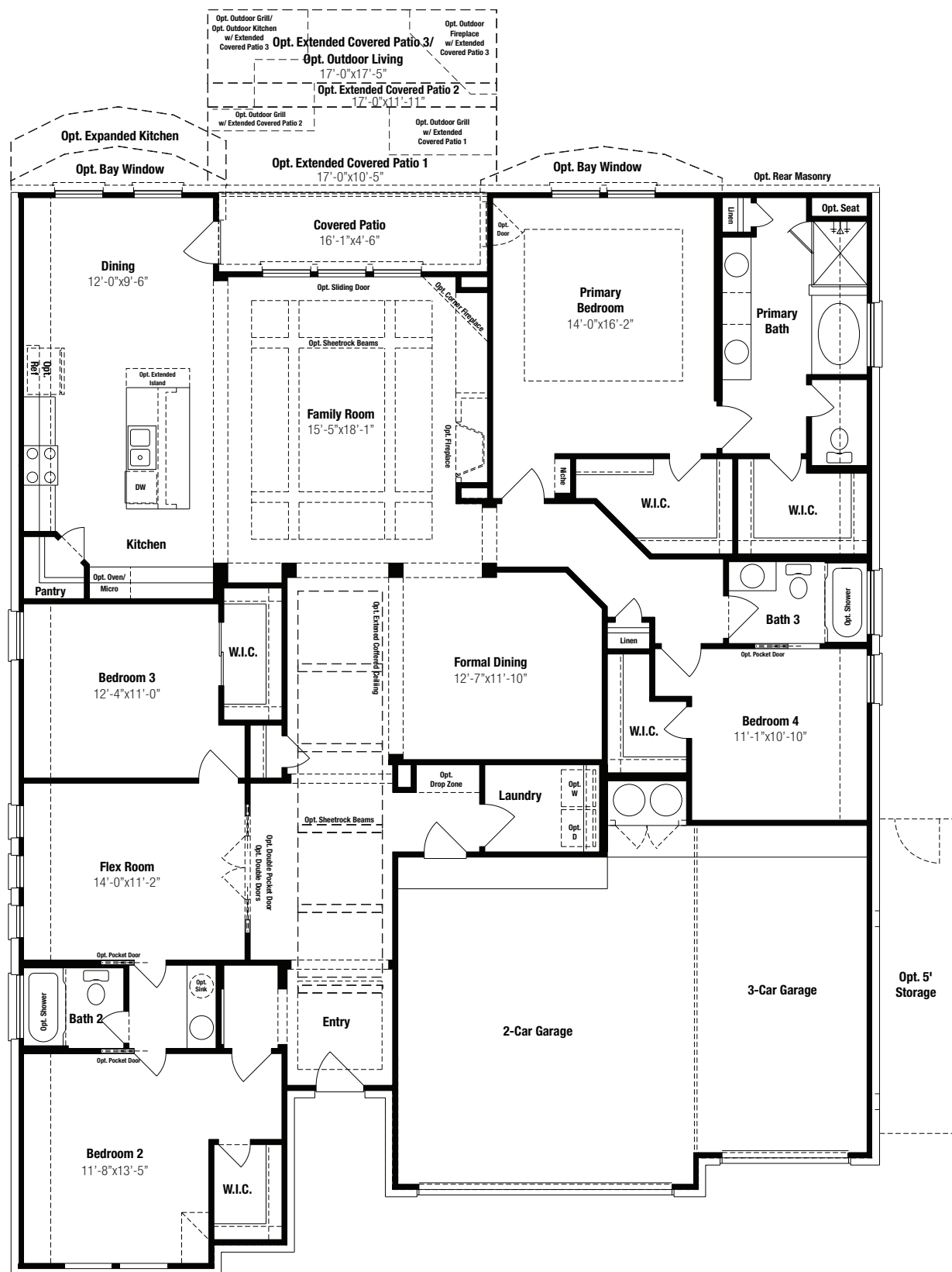
FIRST FLOOR
