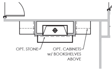
4 - CABINETS @ FIREPLACE #1
