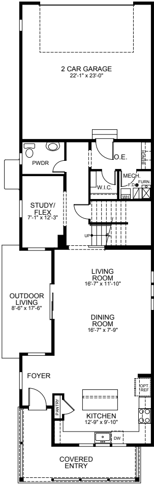
FIRST FLOOR
