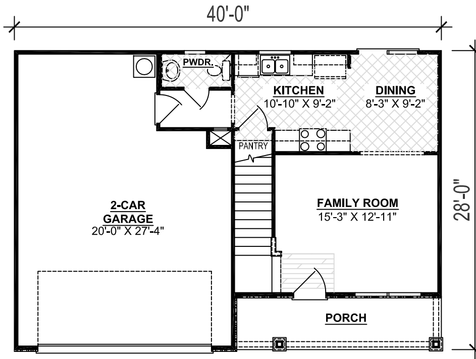
First Floor
