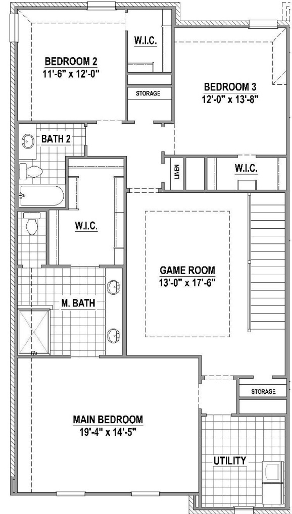
2 nd Floor
