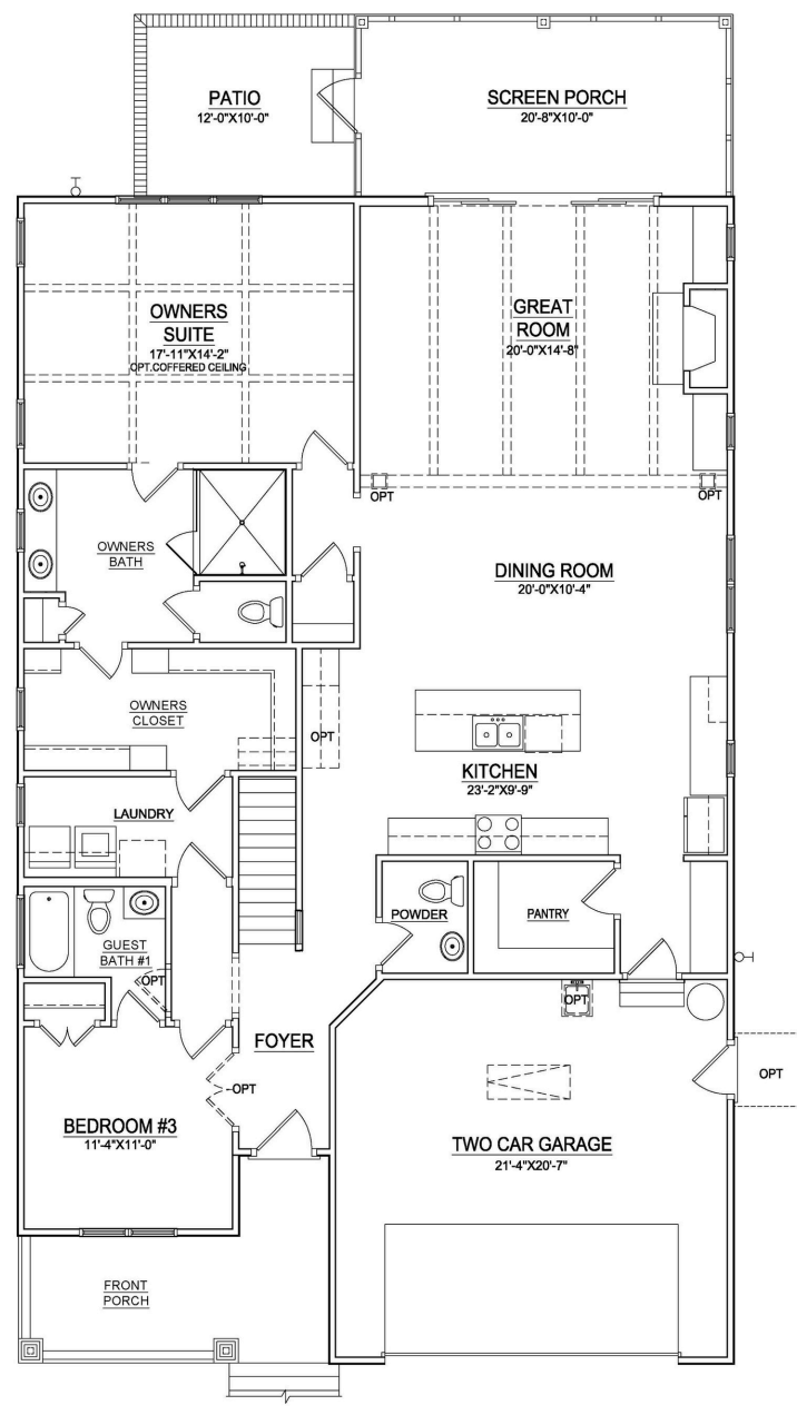
OPT. 1ST FLOOR PLAN W/ SECOND FLOOR
