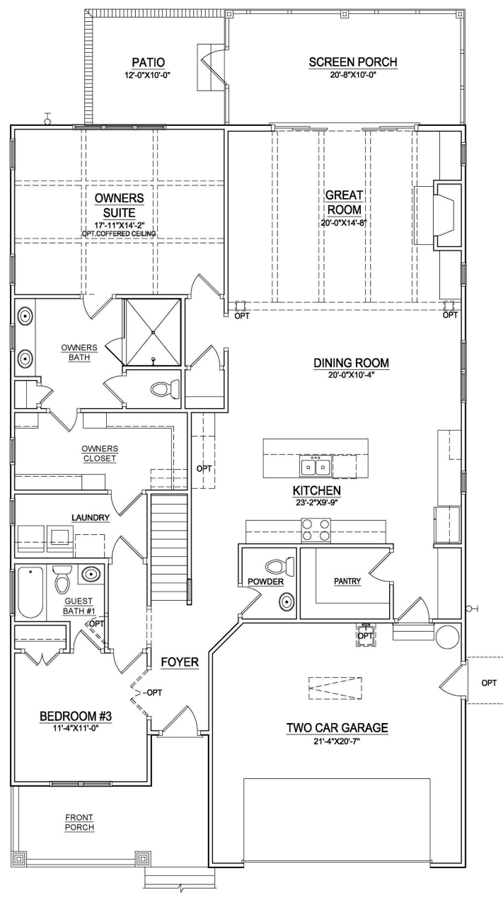
OPT. 1ST FLOOR PLAN W/ SECOND FLOOR
