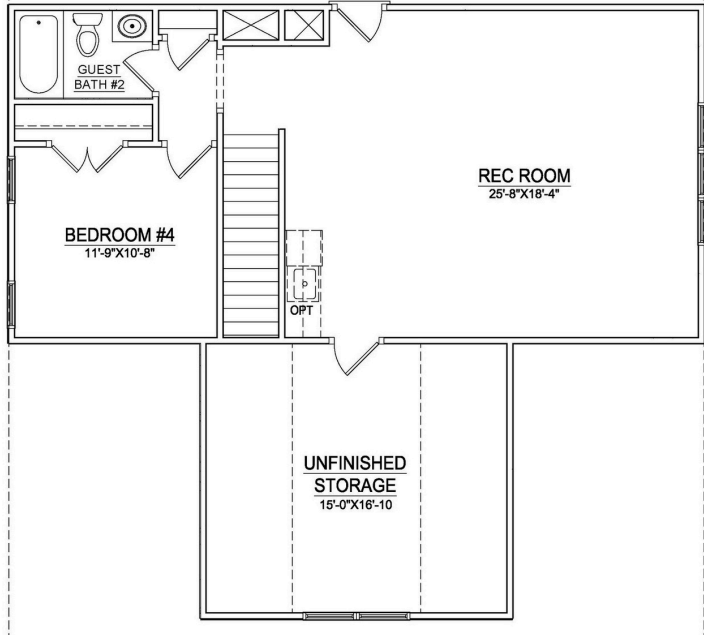
Optional 2nd Floor - Elevation B
