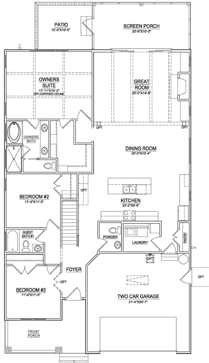
1ST FLOOR PLAN W/ SECOND FLOOR
