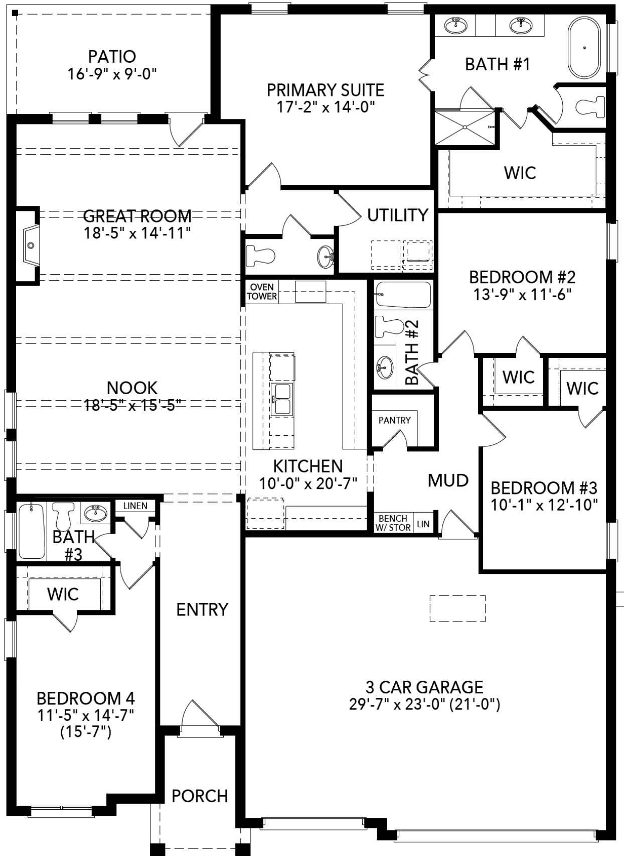
First Floor
