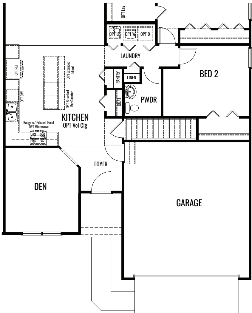
OPTIONAL LAUNDRY TUB (at slab)
