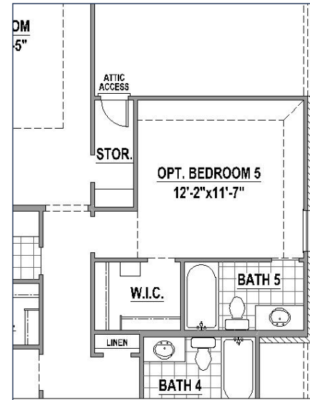
Bedroom 5 w/ Bath 5 (+279 SF)
