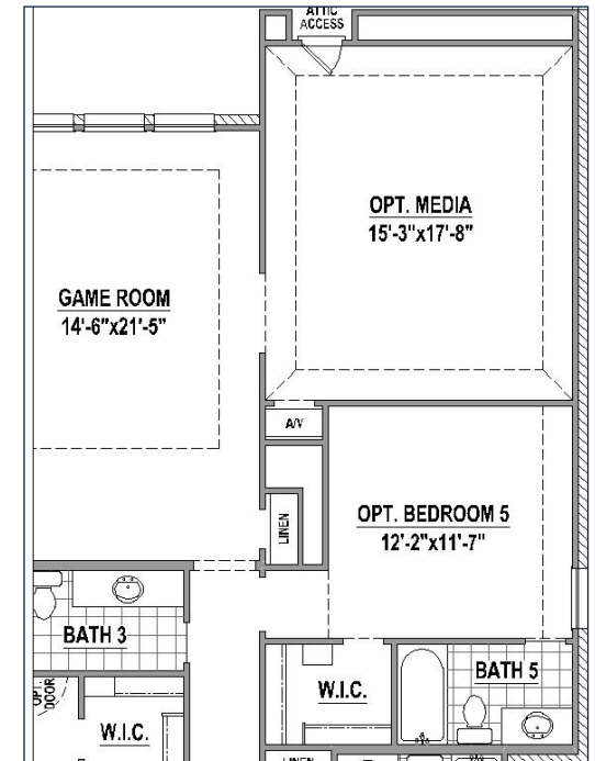
Bedroom 5, Bath 5 & Media Room (+568 SF)
