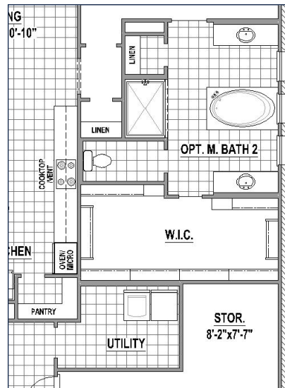
Alternate Main Bath Layout 2 w/ Storage ILO Tandem Garage (+81 SF)
