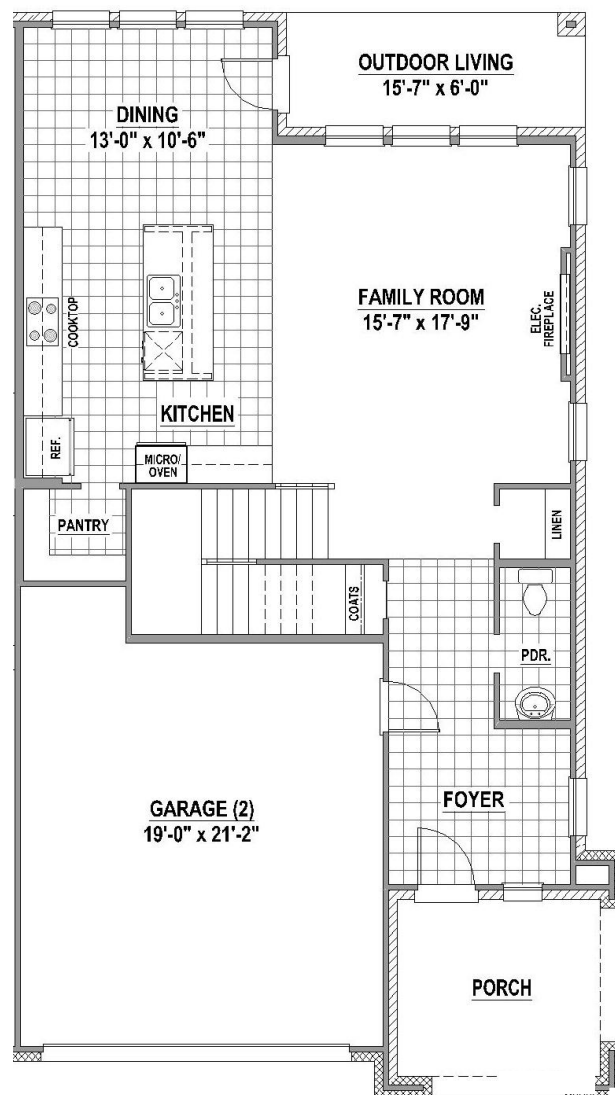
1 st Floor
