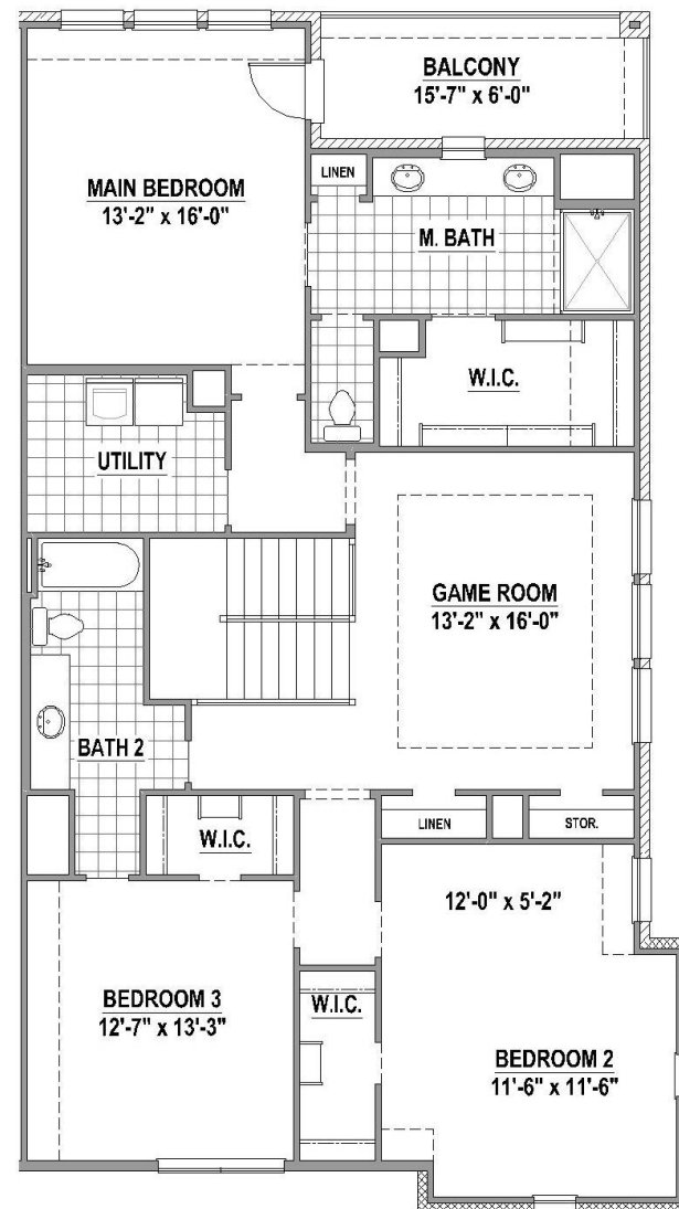
2 nd Floor
