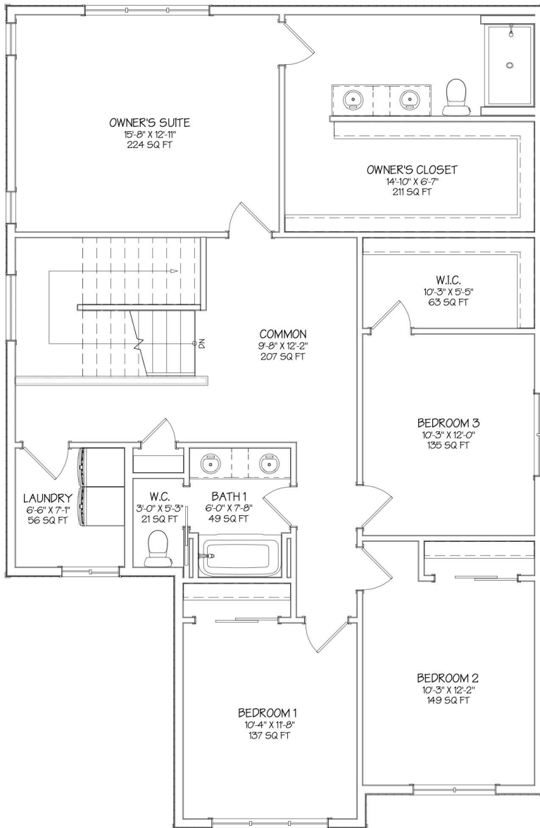
Riviera 2.0 - Base Plan - Upper Floor - 1,390 sq ft
