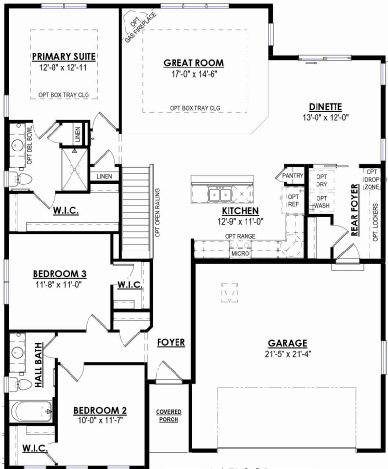
1st FLOOR 1,717 Sq. Ft.
