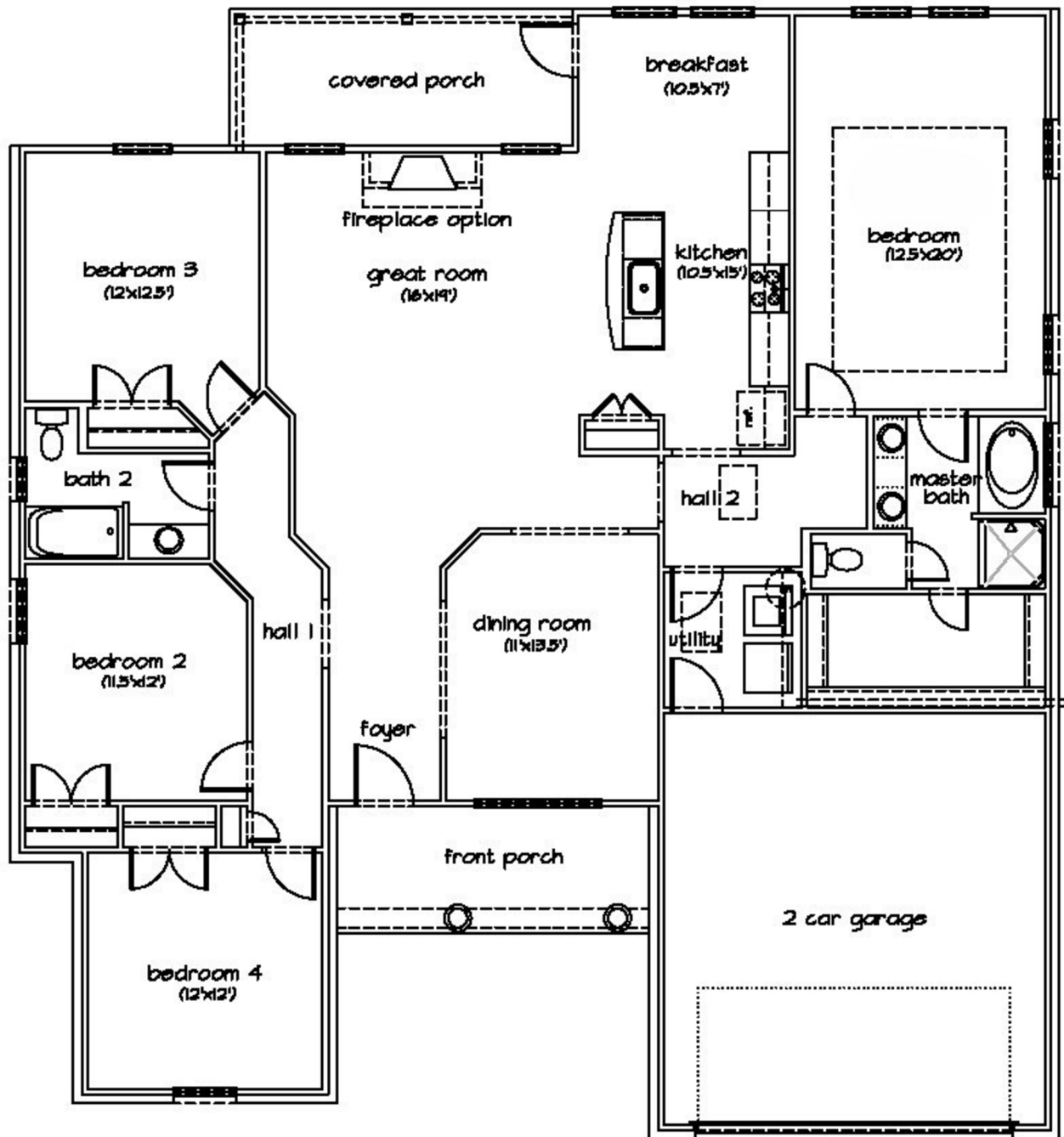
FLOOR PLAN (53'-11"x57'-10")
