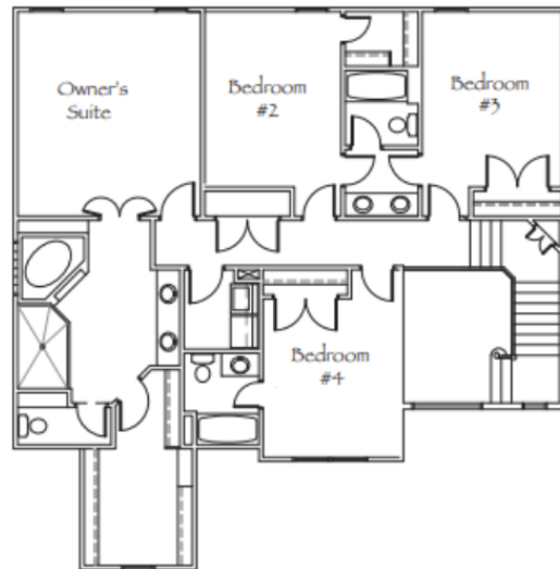
2nd Floor Plan 1449 sq ft
