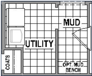
Optional Mud Bench
