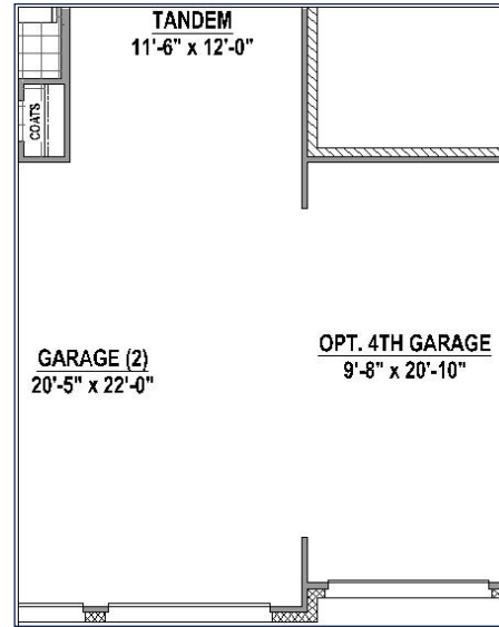
Optional 4th Car Garage
