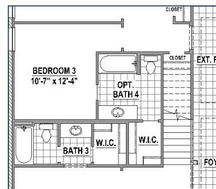
Bath 4 w/ Stairs to 2nd Floor Options
