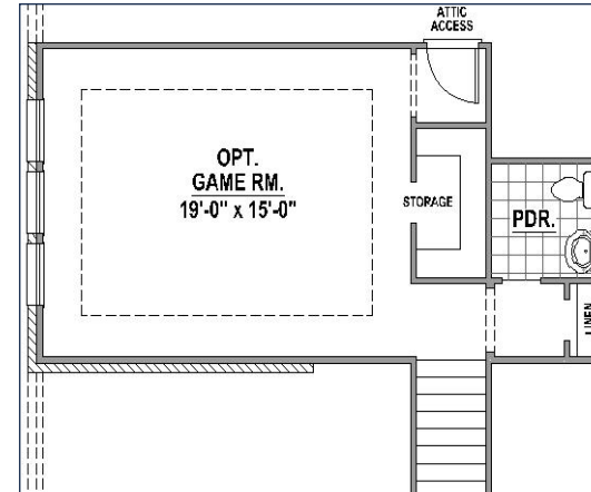
Game Room & Powder Bath (+441 SF)
