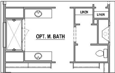
Optional Main Bath Layout
