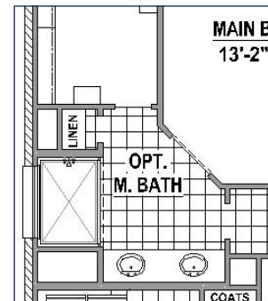
Optional Main Bath Layout
