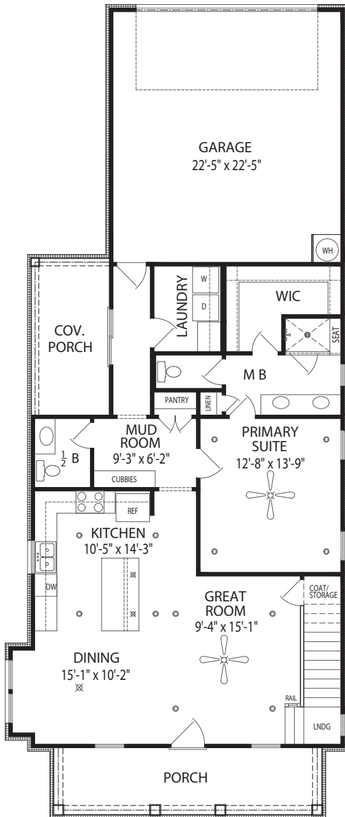
First Level
