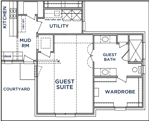
GUEST SUITE AND BATH OPTION in lieu of One Car Garage
